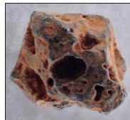
Enlarged photo of fuel debris sample (second retrieval) (Source: JAEA/TEPCO)
